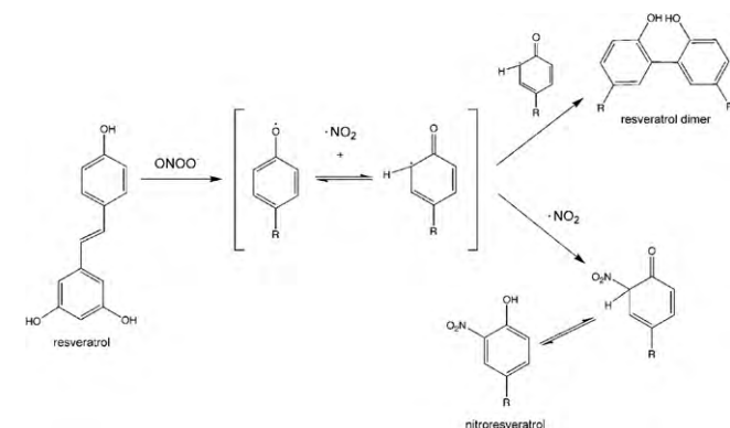
Fig. 6. Hypothetical pathway for nitroresveratrol and resveratrol dimer formation by peroxynitrite.
